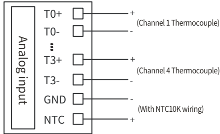
Figure 14 Customized 43C thermocouple wiring
