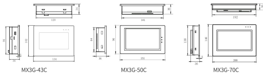
Figure 1 Installation dimension
